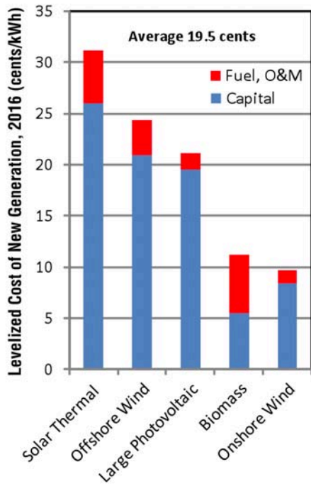
Figure 4. Levelized Cost of New Renewable Power-Only Generation Resources On Line in 2016. (3)
