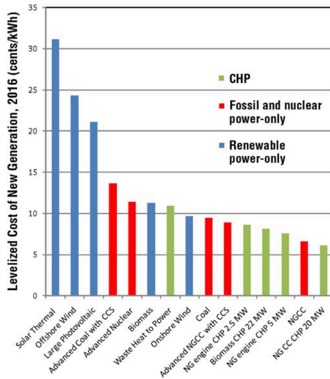
Figure 8. Summary of Levelized Cost of Generation Resources On Line in 2016. (6)
