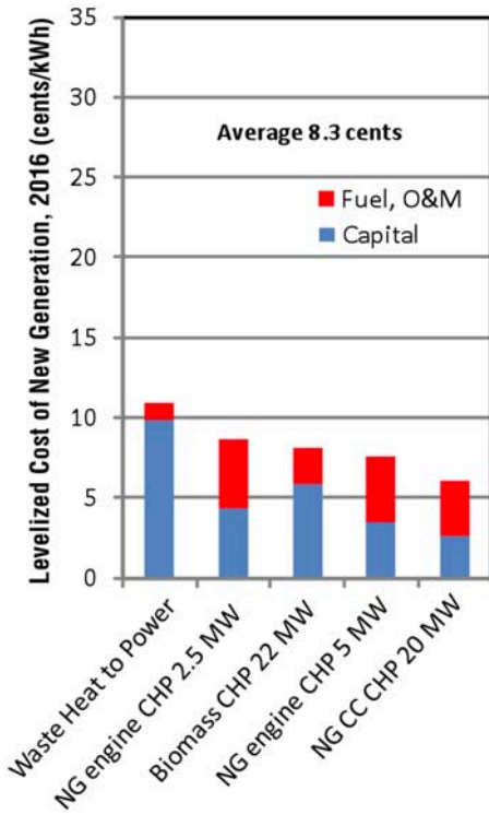
Figure 7. Levelized Cost of New Combined Heat and Power Generation Resources On Line in 2016. (5)
