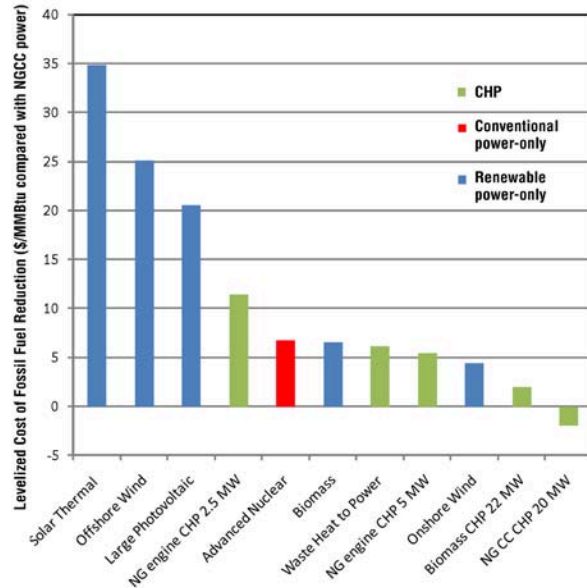
Figure 9. Levelized Cost of Power Generation Fossil Fuel Reduction Compared With Natural Gas Combined-Cycle On Line in 2016. (8)
