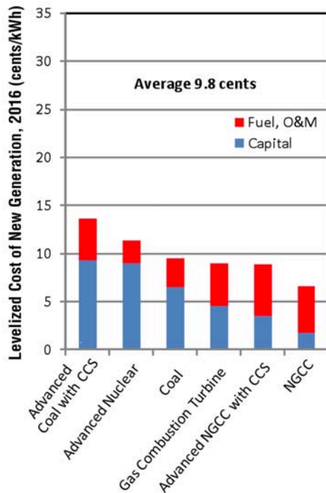
Figure 5. Levelized Cost of New Nonrenewable Power-Only Generation Resources On Line in 2016. (3)
