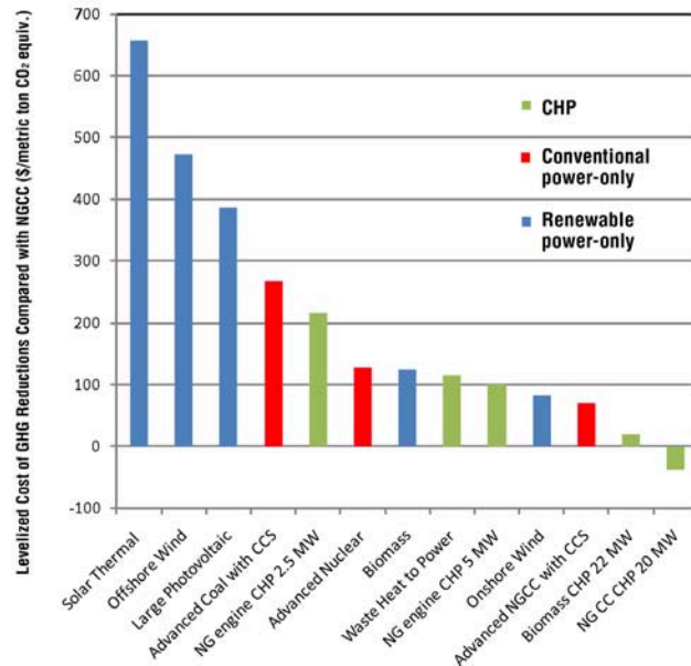
Figure 10. Levelized Cost of Greenhouse Gas Reduction for New Generation Resources Compared With Natural Gas Combined-Cycle On Line in 2016. (8)
